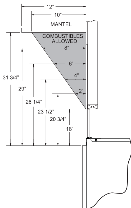
Figure 2 - Mantel Clearances
